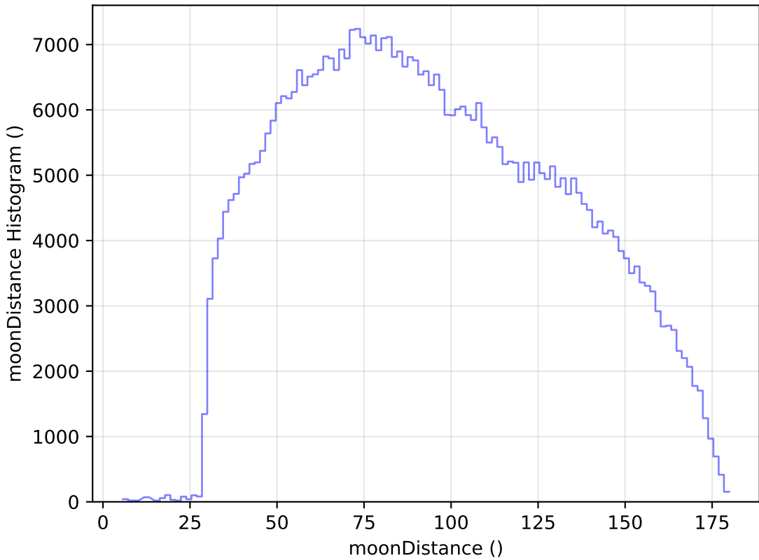
internal_u_expt38_nscale1.0v3.4_10yrs All sky i band: moonDistance Histogram
