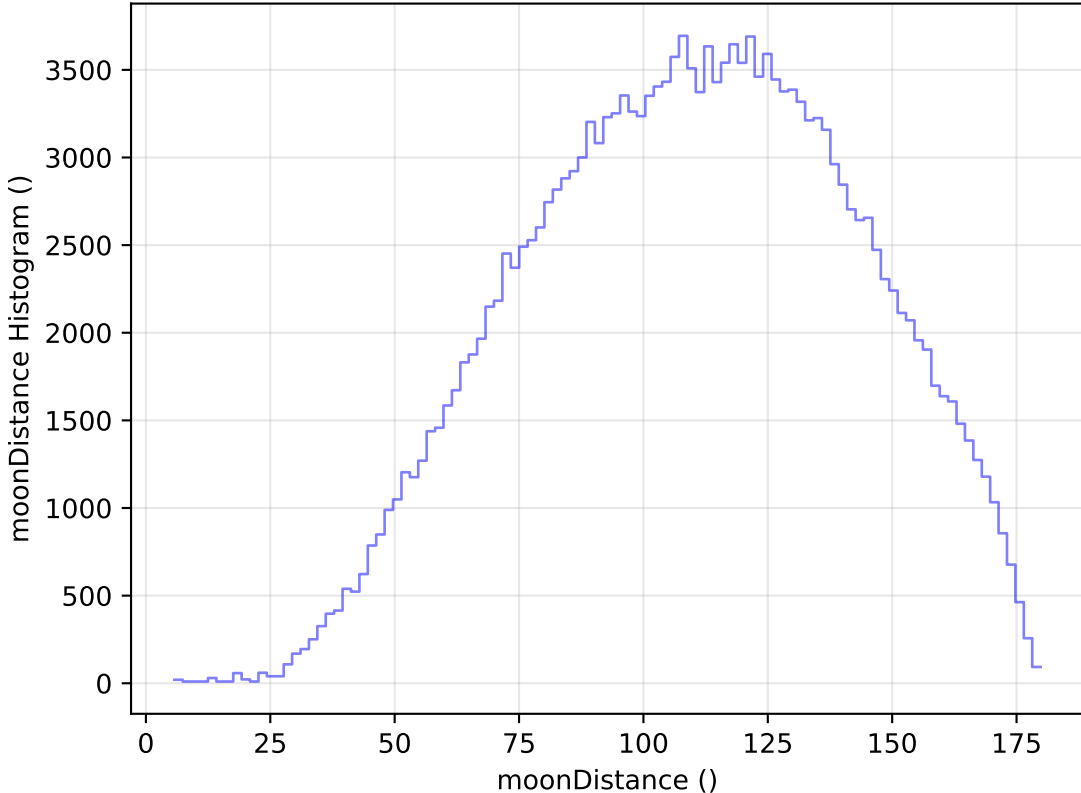
internal_u_expt38_nscale1.0v3.4_10yrs All sky g band: moonDistance Histogram
