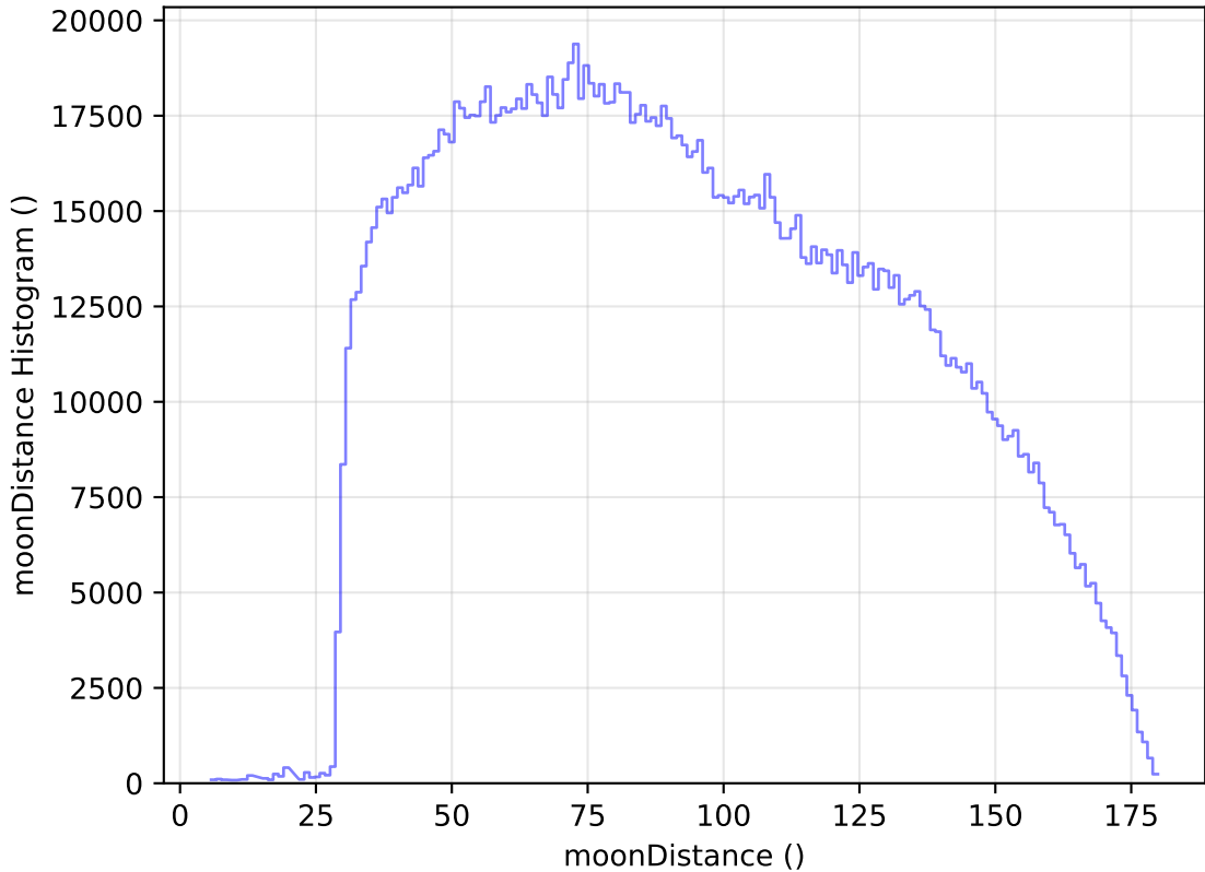
internal_u_expt38_nscale1.0v3.4_10yrs All sky all bands: moonDistance Histogram
