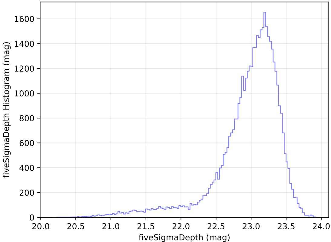
internal_u_expt38_nscale1.0v3.4_10yrs Yr 1 z band: fiveSigmaDepth Histogram
