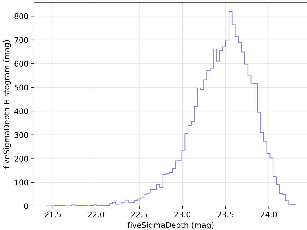
internal_u_expt38_nscale1.0v3.4_10yrs Yr 1 u band: fiveSigmaDepth Histogram
