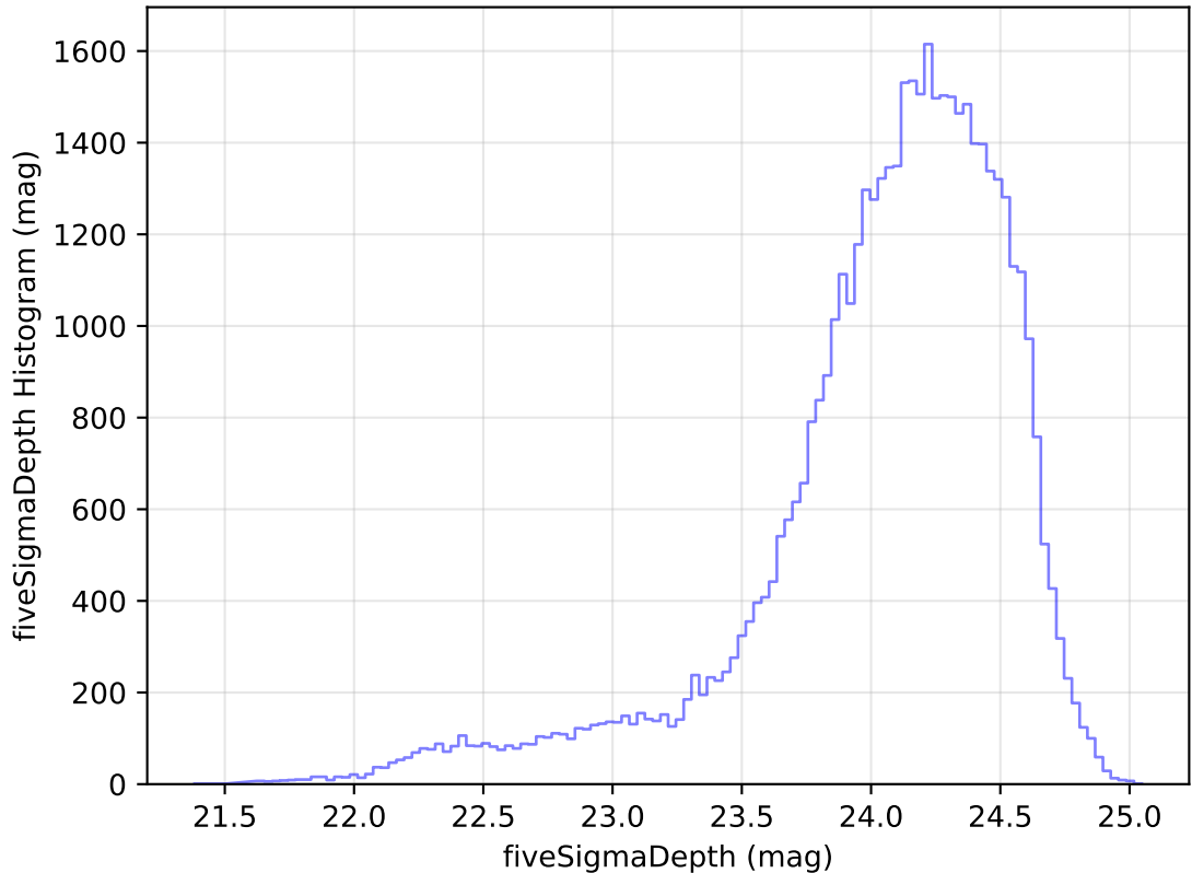
internal_u_expt38_nscale1.0v3.4_10yrs Yr 1 r band: fiveSigmaDepth Histogram
