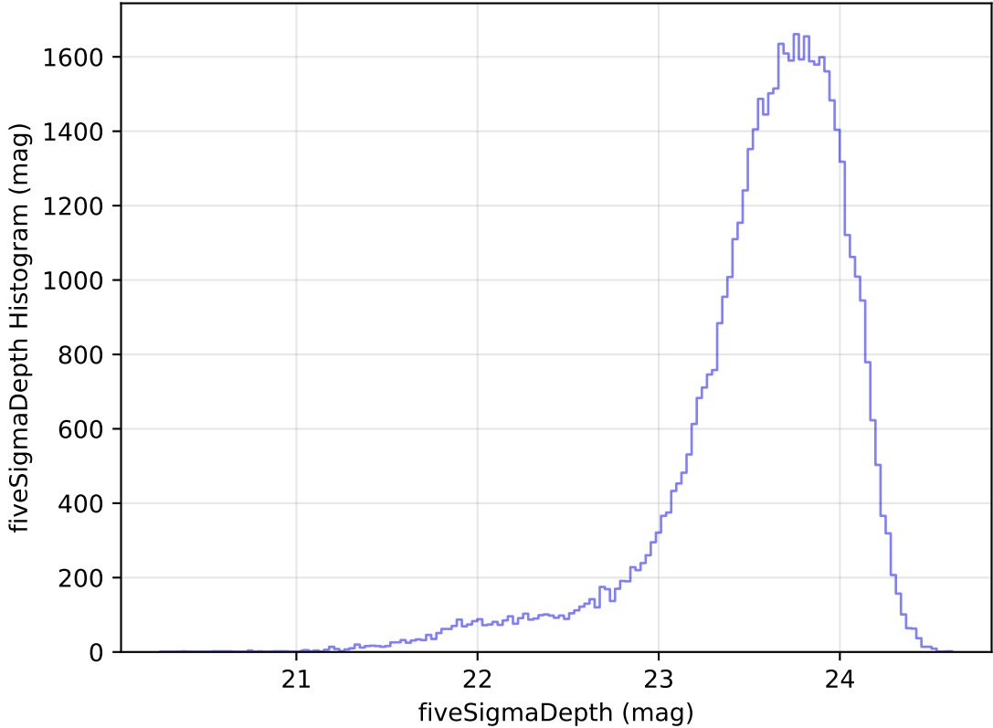
internal_u_expt38_nscale1.0v3.4_10yrs Yr 1 i band: fiveSigmaDepth Histogram
