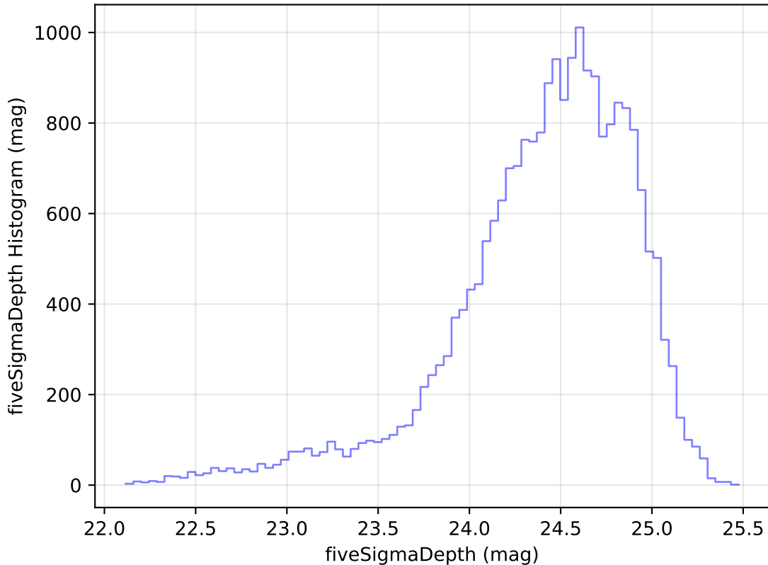
internal_u_expt38_nscale1.0v3.4_10yrs Yr 1 g band: fiveSigmaDepth Histogram
