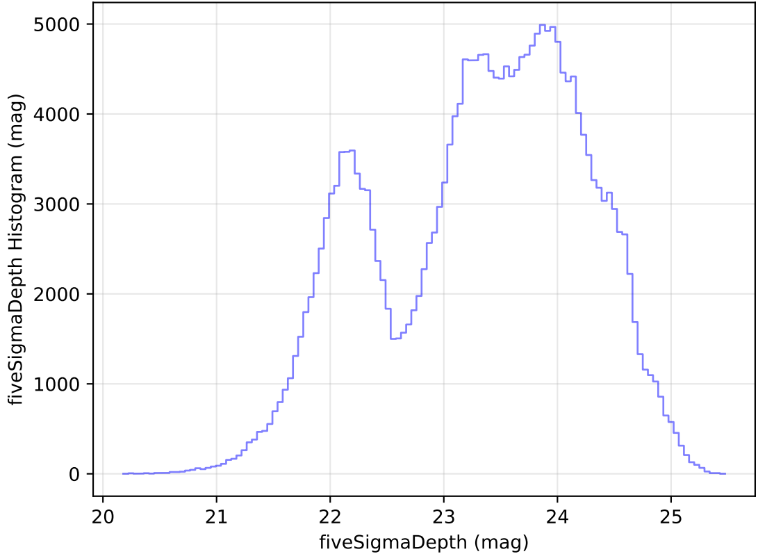
internal_u_expt38_nscale1.0v3.4_10yrs Yr 1 all bands: fiveSigmaDepth Histogram
