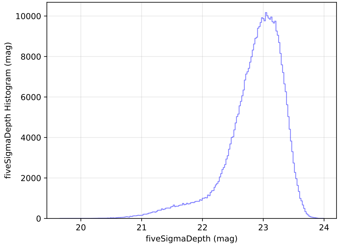
internal_u_expt38_nscale1.0v3.4_10yrs WFD z band: fiveSigmaDepth Histogram
