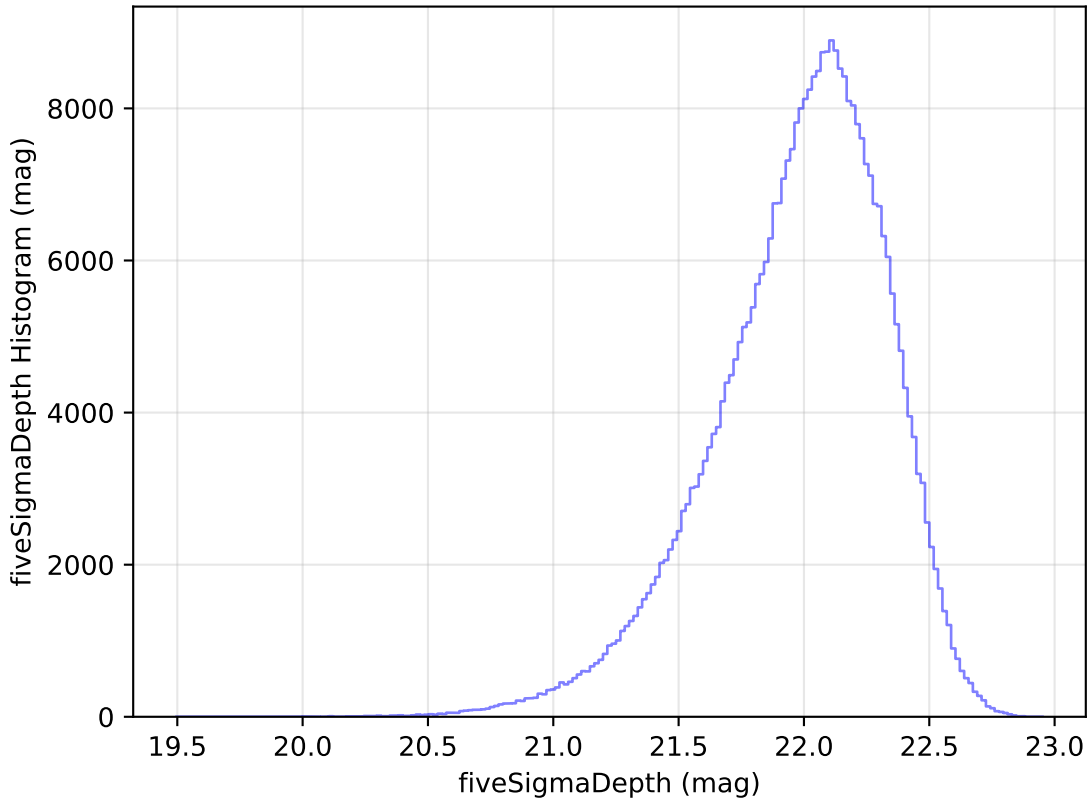
internal_u_expt38_nscale1.0v3.4_10yrs WFD y band: fiveSigmaDepth Histogram
