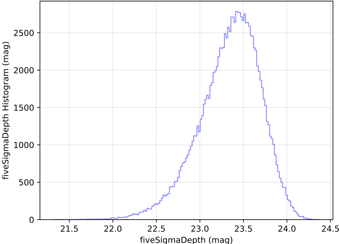
internal_u_expt38_nscale1.0v3.4_10yrs WFD u band: fiveSigmaDepth Histogram
