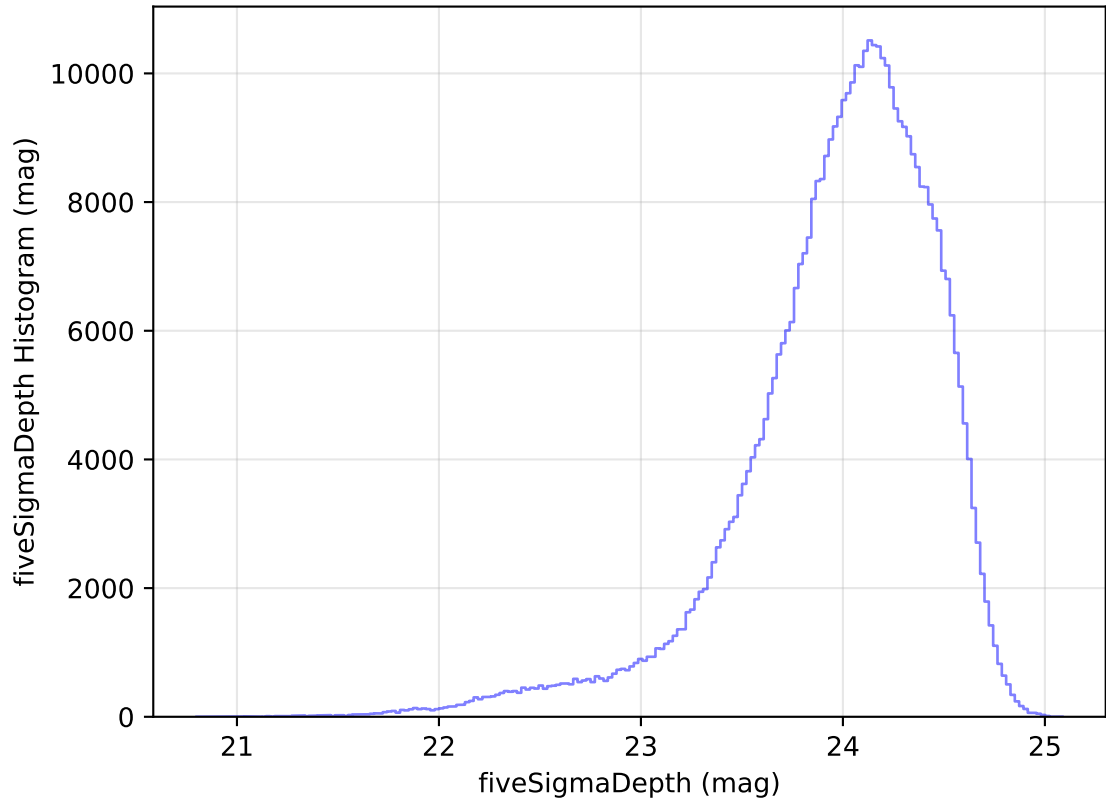
internal_u_expt38_nscale1.0v3.4_10yrs WFD r band: fiveSigmaDepth Histogram
