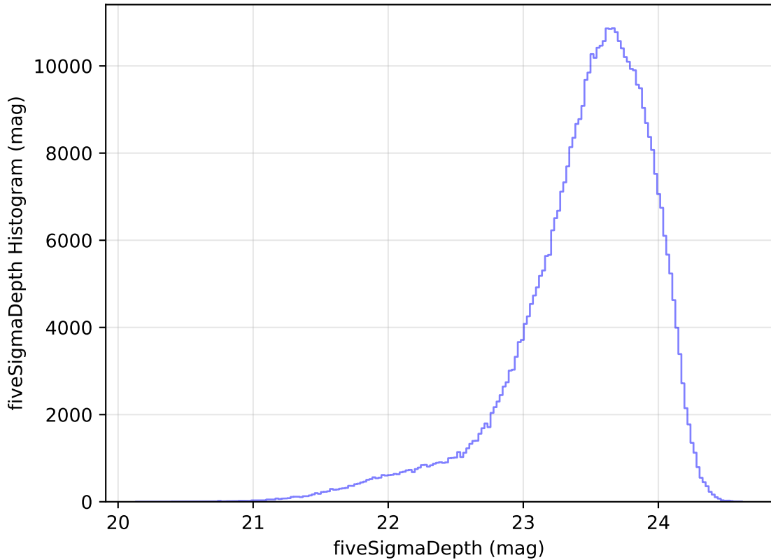
internal_u_expt38_nscale1.0v3.4_10yrs WFD i band: fiveSigmaDepth Histogram
