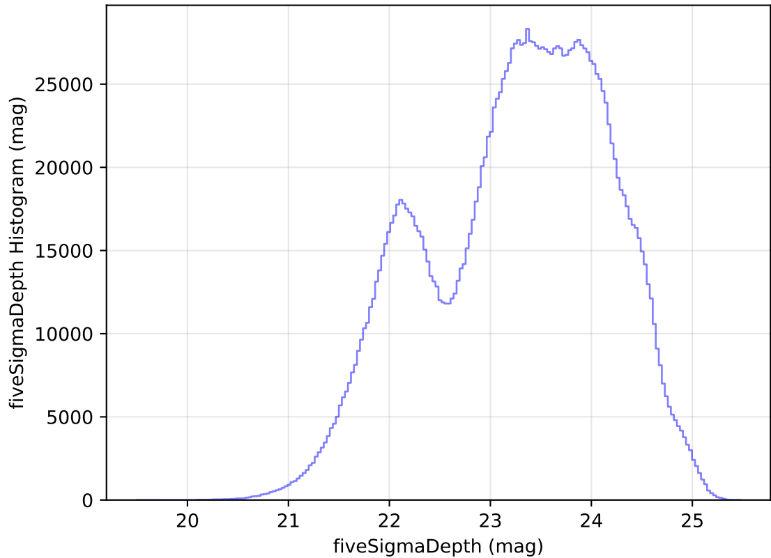
internal_u_expt38_nscale1.0v3.4_10yrs WFD all bands: fiveSigmaDepth Histogram
