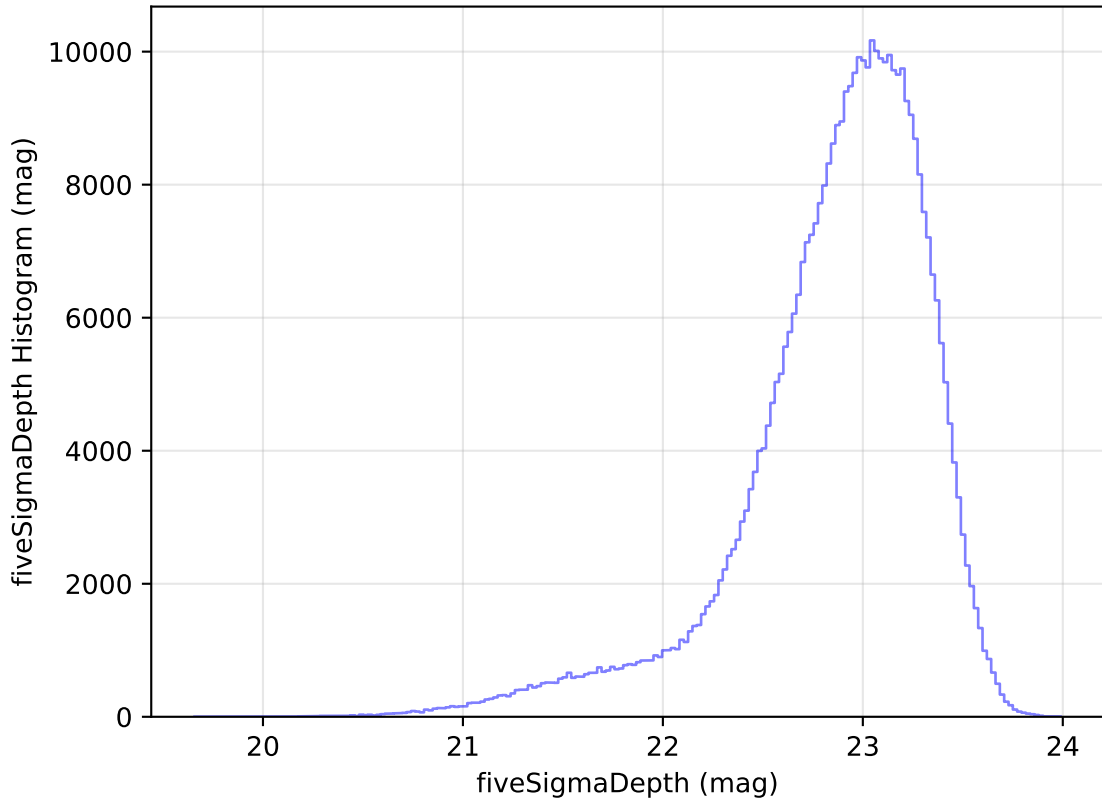
internal_u_expt38_nscale1.0v3.4_10yrs All sky z band: fiveSigmaDepth Histogram
