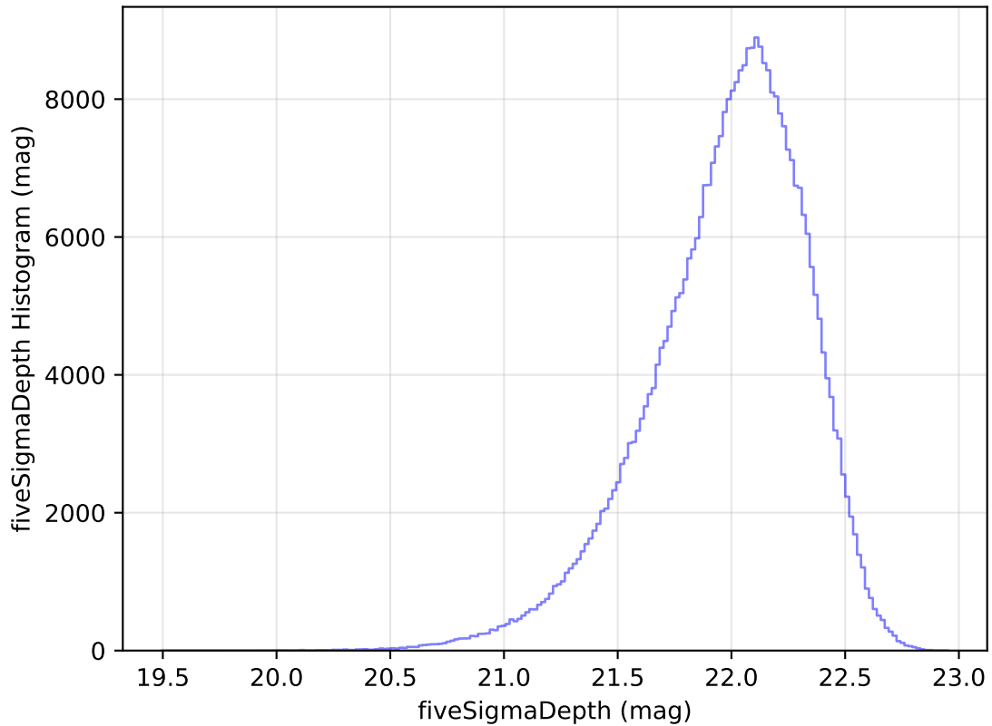
internal_u_expt38_nscale1.0v3.4_10yrs All sky y band: fiveSigmaDepth Histogram
