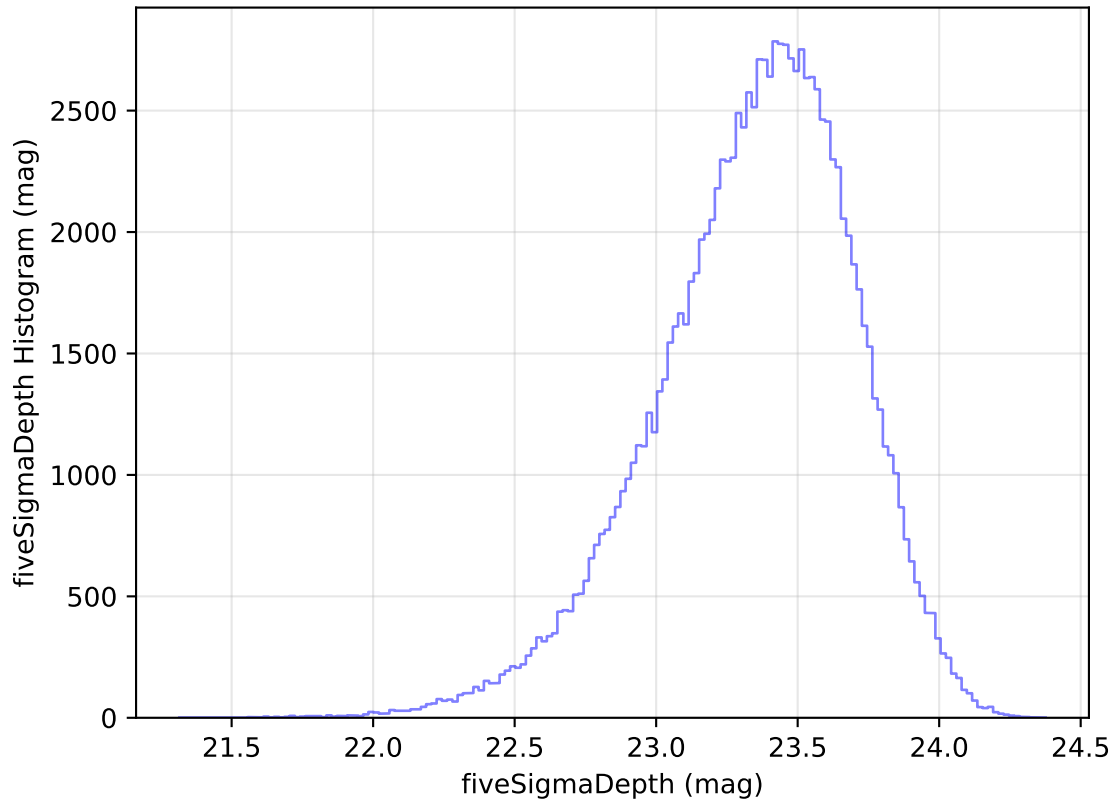
internal_u_expt38_nscale1.0v3.4_10yrs All sky u band: fiveSigmaDepth Histogram
