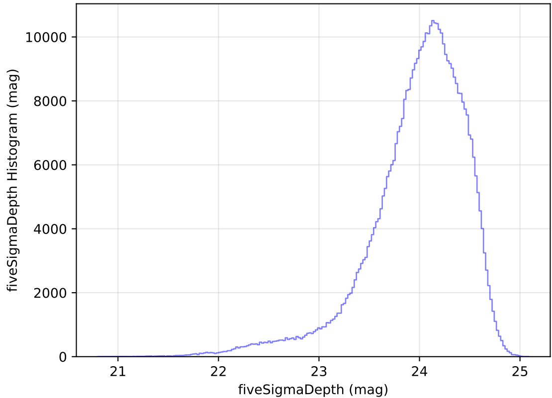
internal_u_expt38_nscale1.0v3.4_10yrs All sky r band: fiveSigmaDepth Histogram
