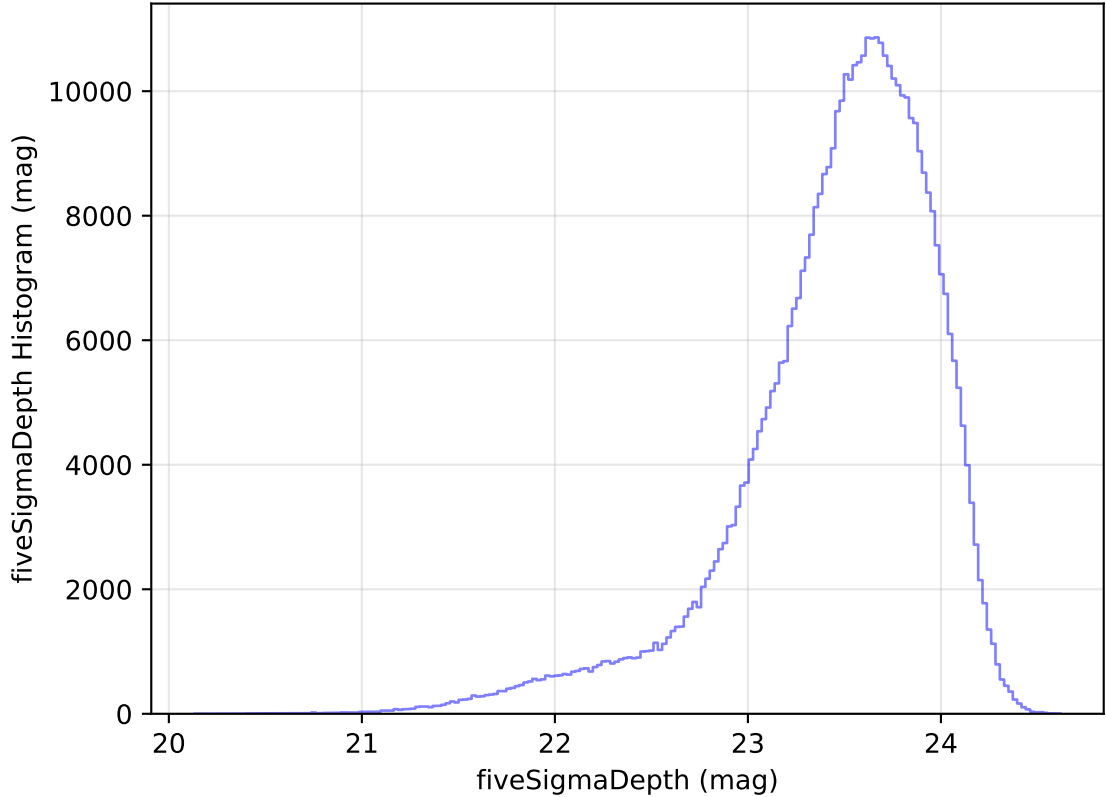
internal_u_expt38_nscale1.0v3.4_10yrs All sky i band: fiveSigmaDepth Histogram
