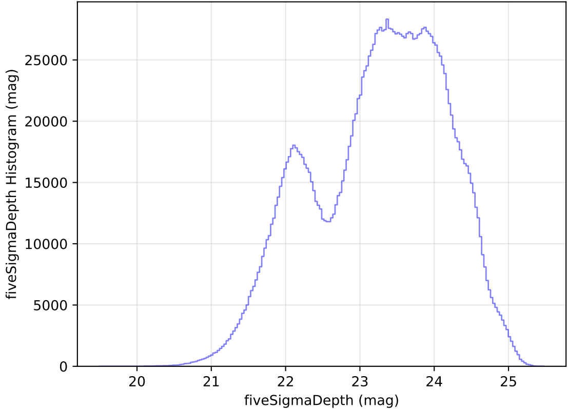
internal_u_expt38_nscale1.0v3.4_10yrs All sky all bands: fiveSigmaDepth Histogram
