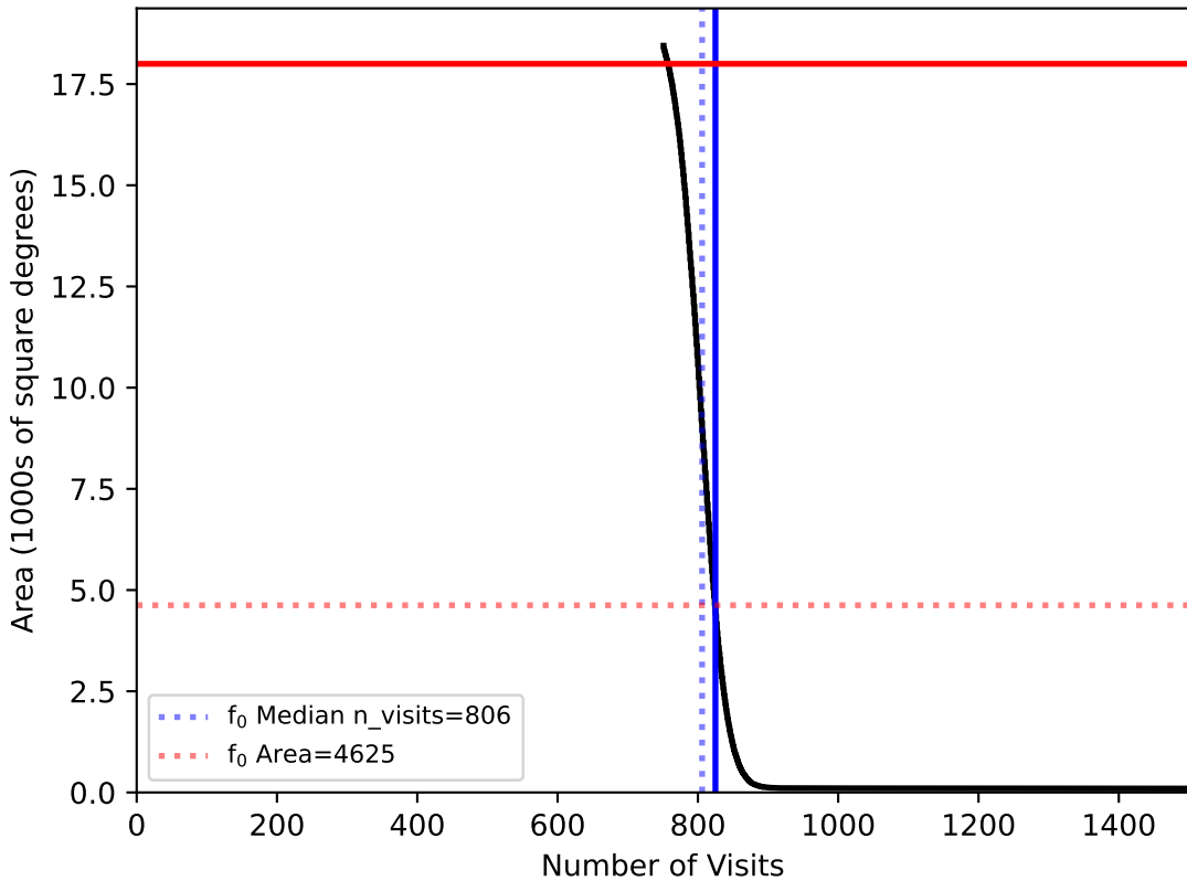
internal_u_expt38_nscale1.0v3.4_10yrs WFD: fO
