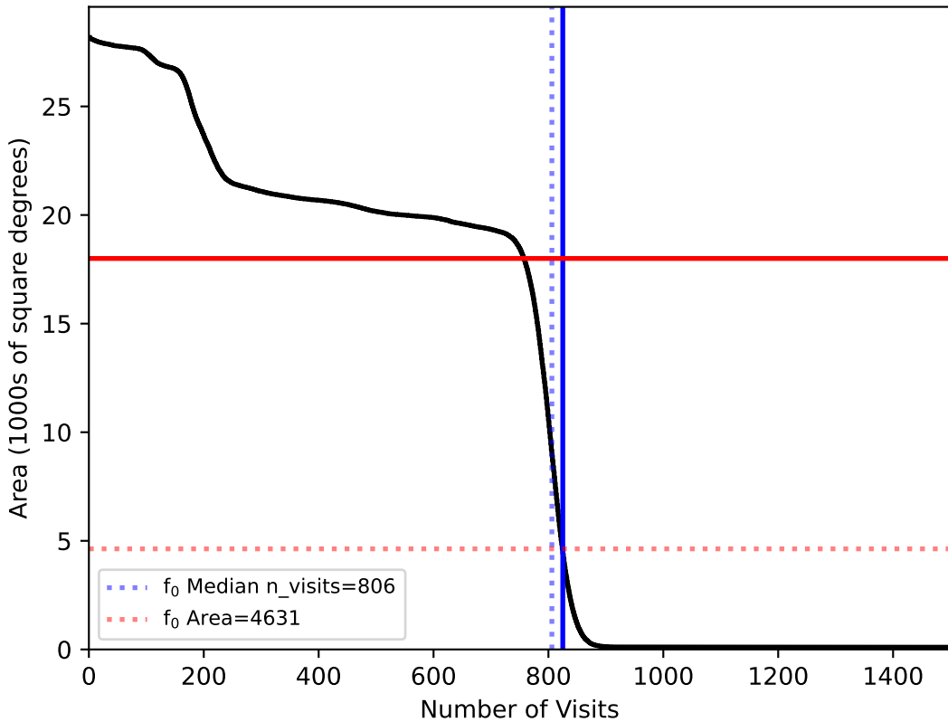
internal_u_expt38_nscale1.0v3.4_10yrs All sky: f0
