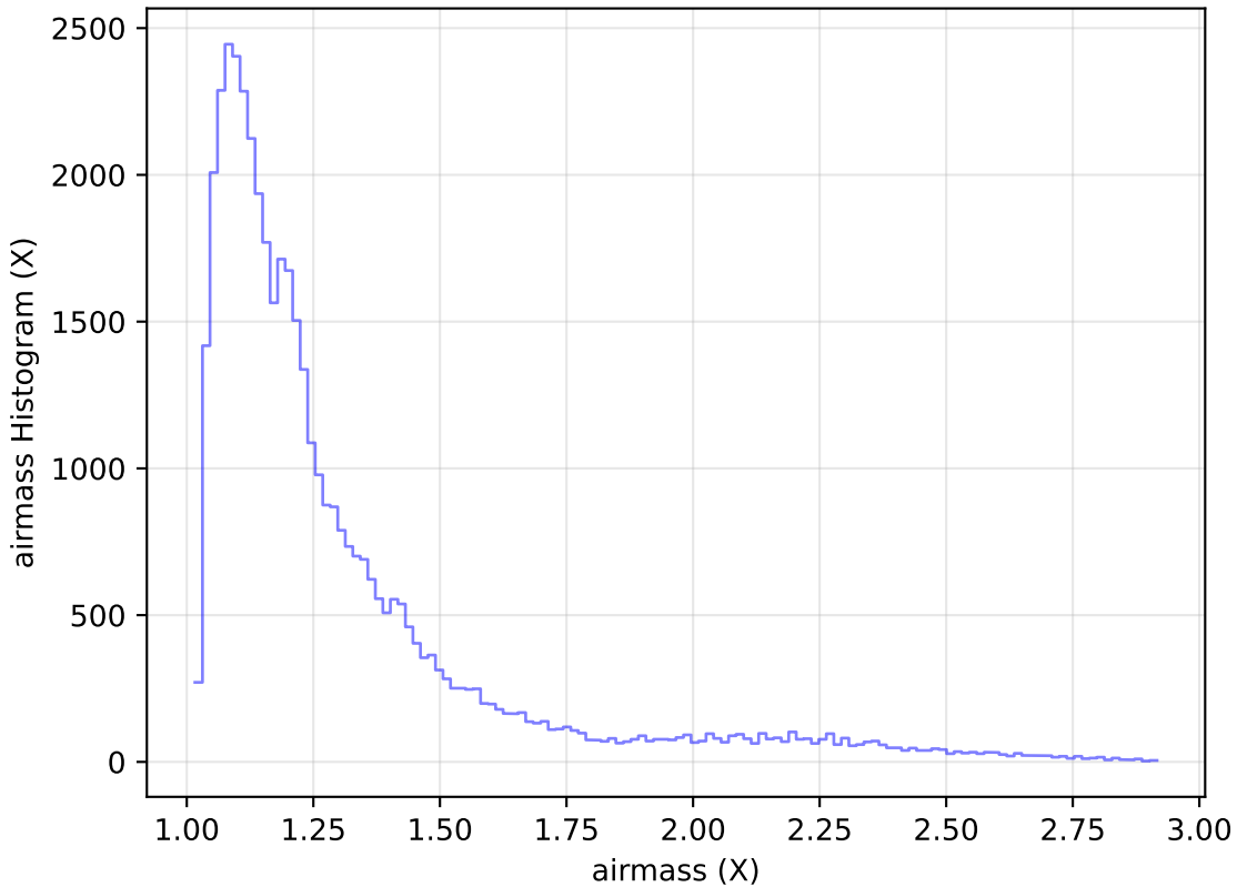
internal_u_expt38_nscale1.0v3.4_10yrs Yr 1 z band: airmass Histogram
