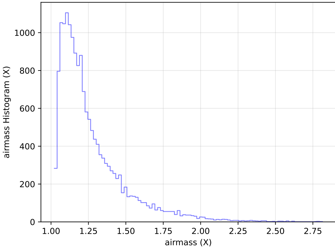
internal_u_expt38_nscale1.0v3.4_10yrs Yr 1 u band: airmass Histogram
