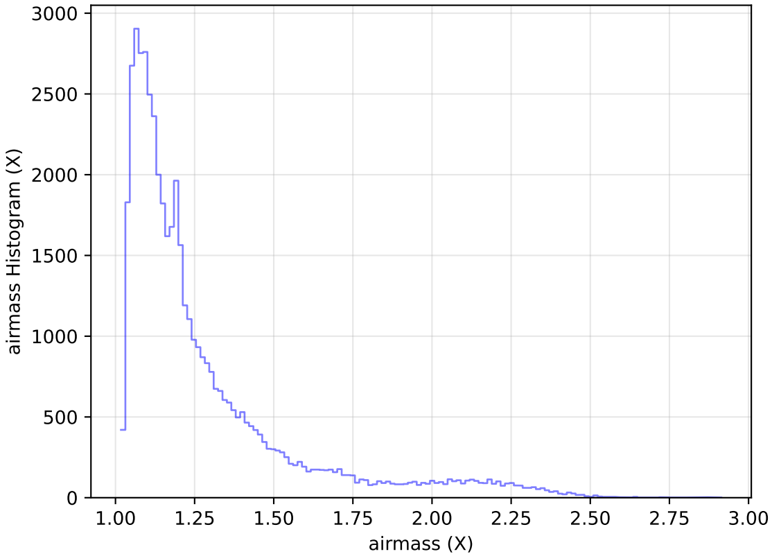
internal_u_expt38_nscale1.0v3.4_10yrs Yr 1 r band: airmass Histogram
