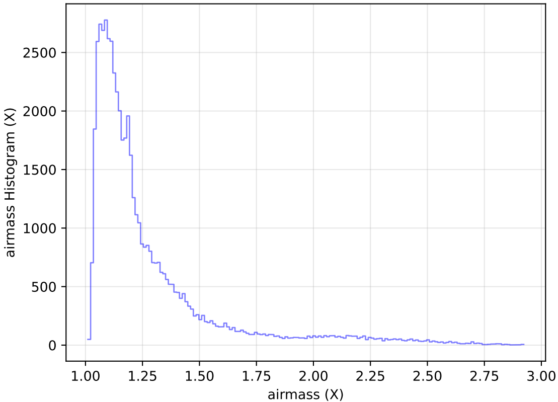
internal_u_expt38_nscale1.0v3.4_10yrs Yr 1 i band: airmass Histogram
