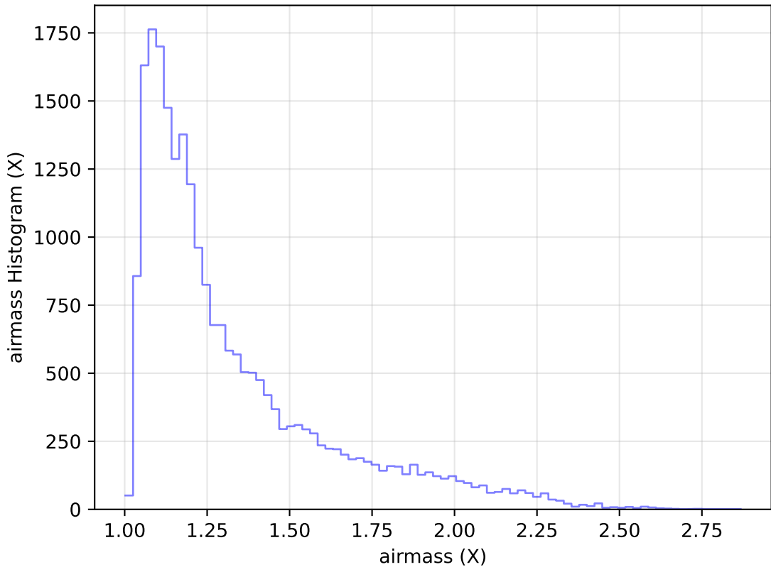
internal_u_expt38_nscale1.0v3.4_10yrs Yr 1 g band: airmass Histogram
