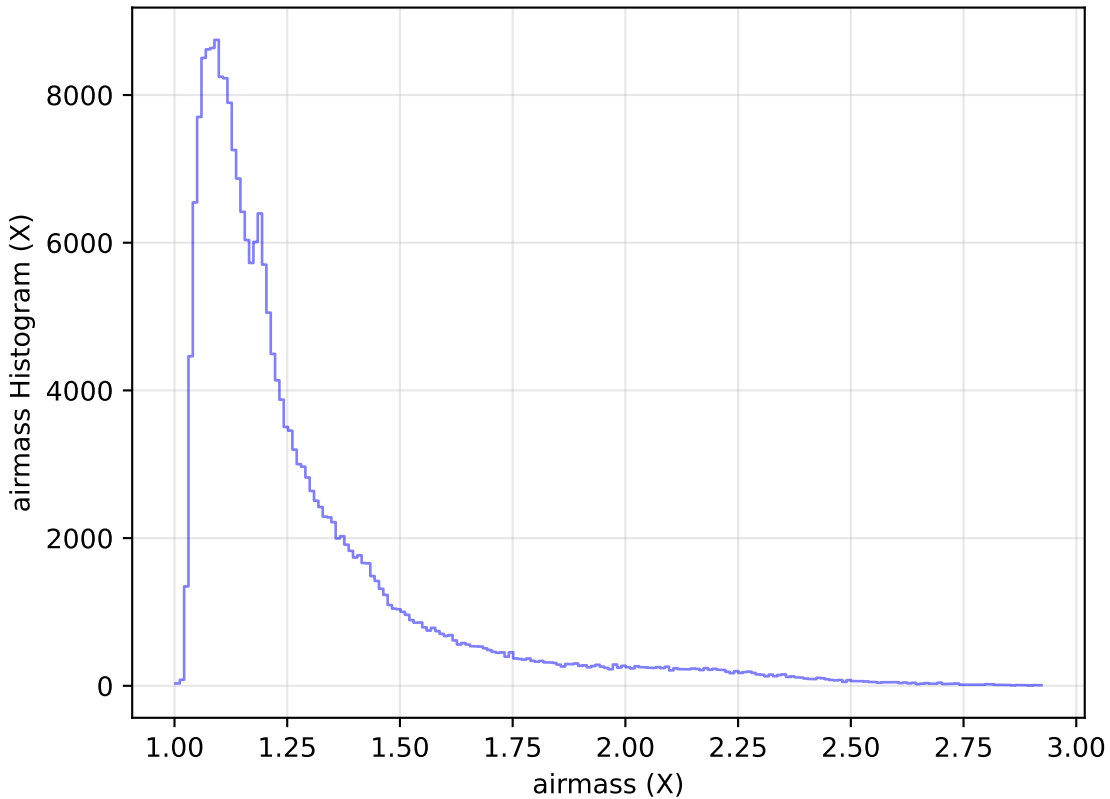
internal_u_expt38_nscale1.0v3.4_10yrs Yr 1 all bands: airmass Histogram
