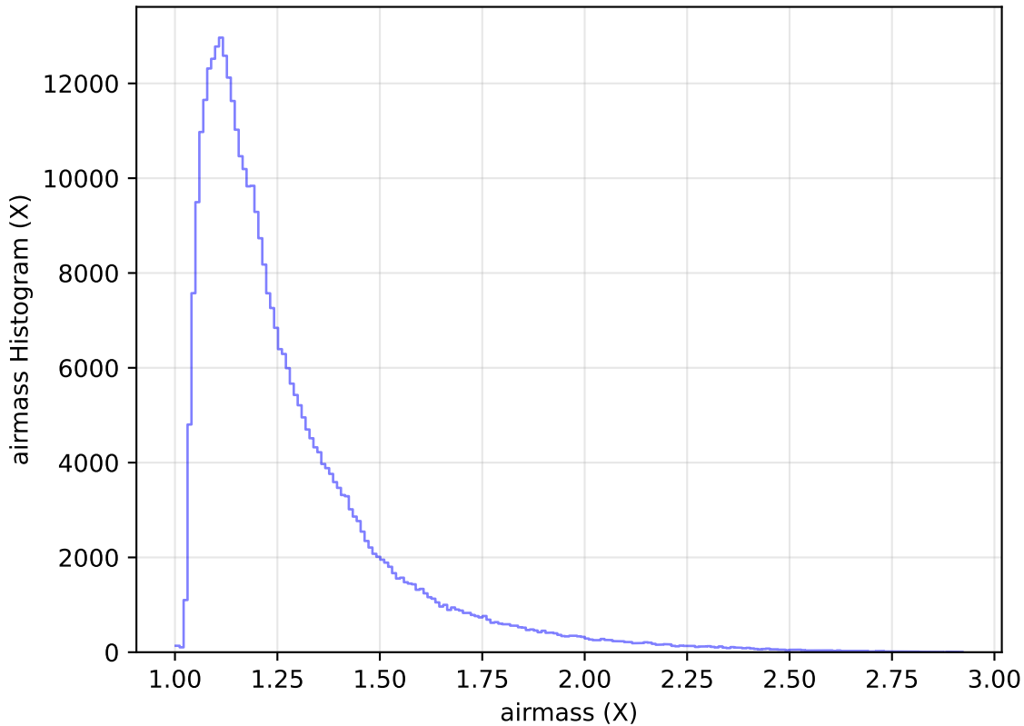
internal_u_expt38_nscale1.0v3.4_10yrs WFD y band: airmass Histogram
