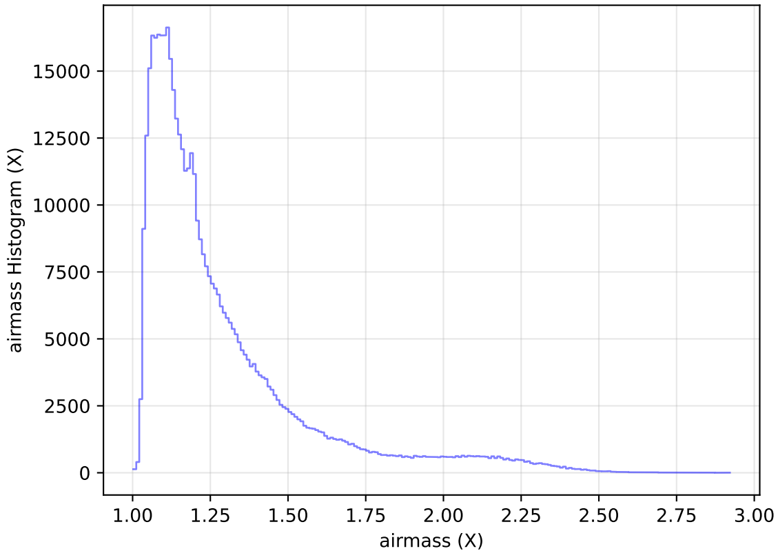
internal_u_expt38_nscale1.0v3.4_10yrs WFD r band: airmass Histogram
