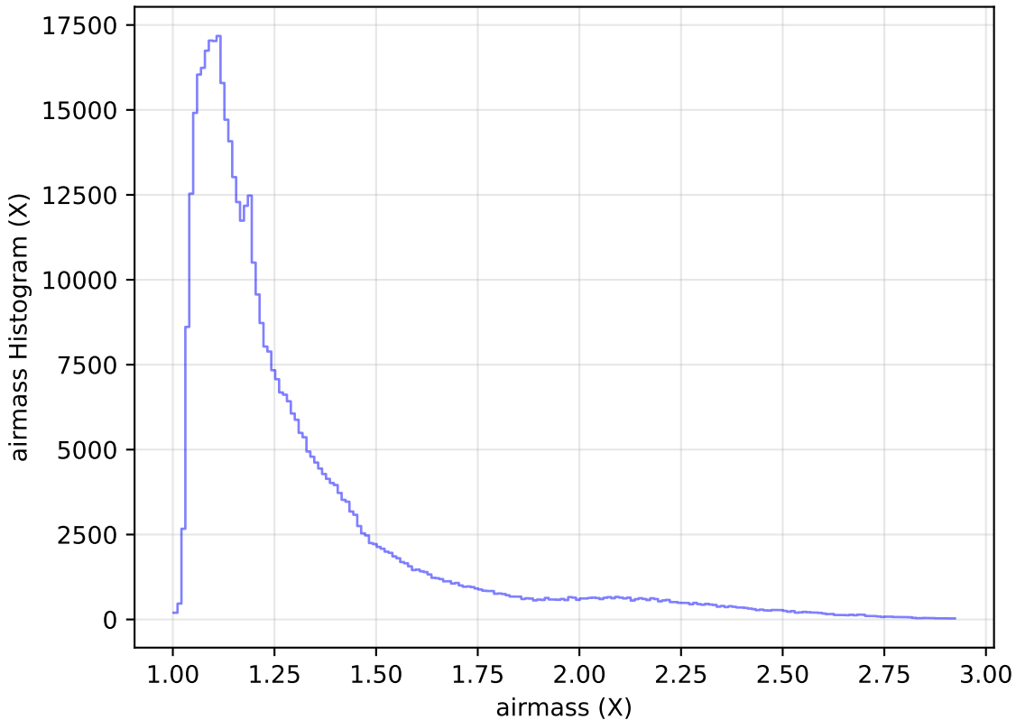
internal_u_expt38_nscale1.0v3.4_10yrs WFD i band: airmass Histogram
