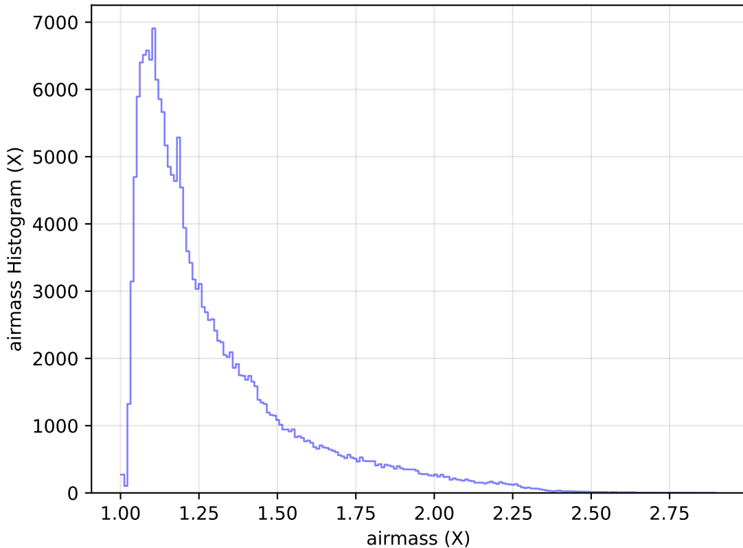
internal_u_expt38_nscale1.0v3.4_10yrs WFD g band: airmass Histogram
