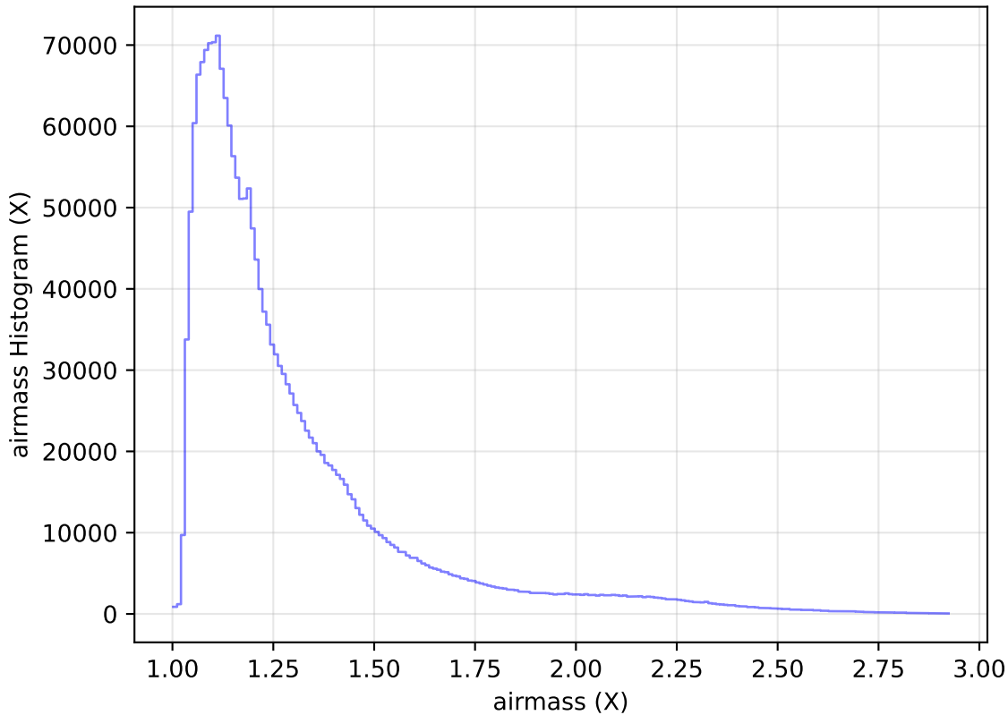
internal_u_expt38_nscale1.0v3.4_10yrs WFD all bands: airmass Histogram
