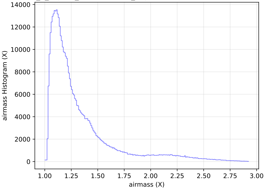
internal_u_expt38_nscale1.0v3.4_10yrs All sky z band: airmass Histogram
