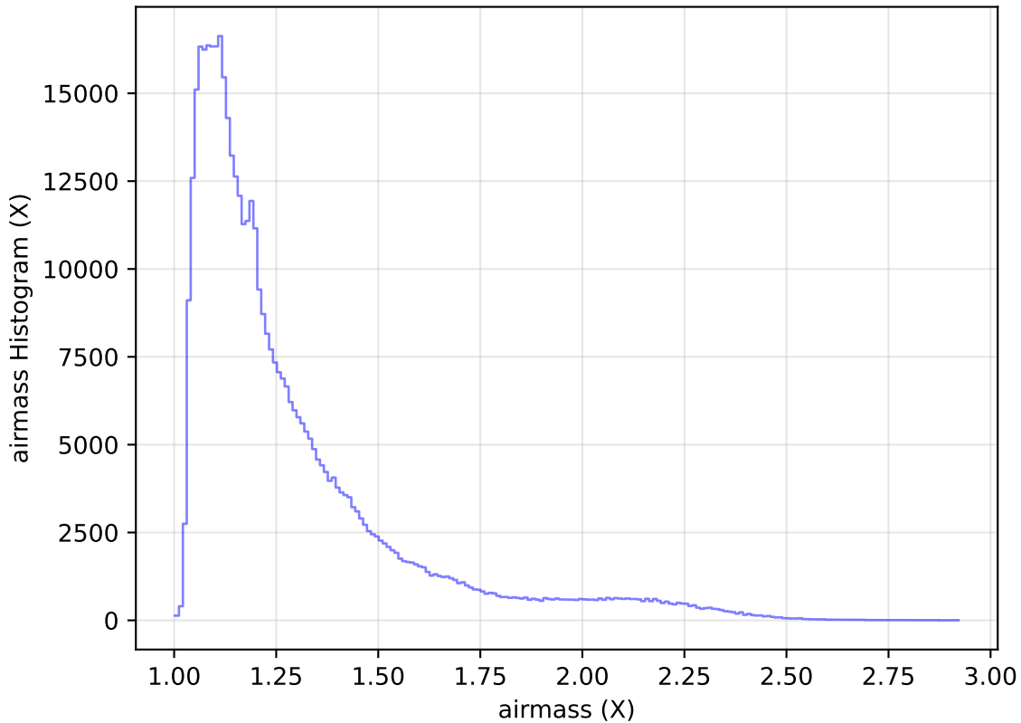
internal_u_expt38_nscale1.0v3.4_10yrs All sky r band: airmass Histogram
