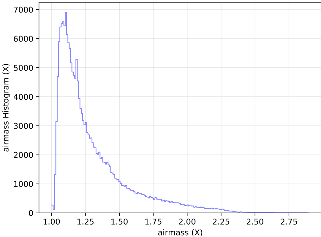
internal_u_expt38_nscale1.0v3.4_10yrs All sky g band: airmass Histogram
