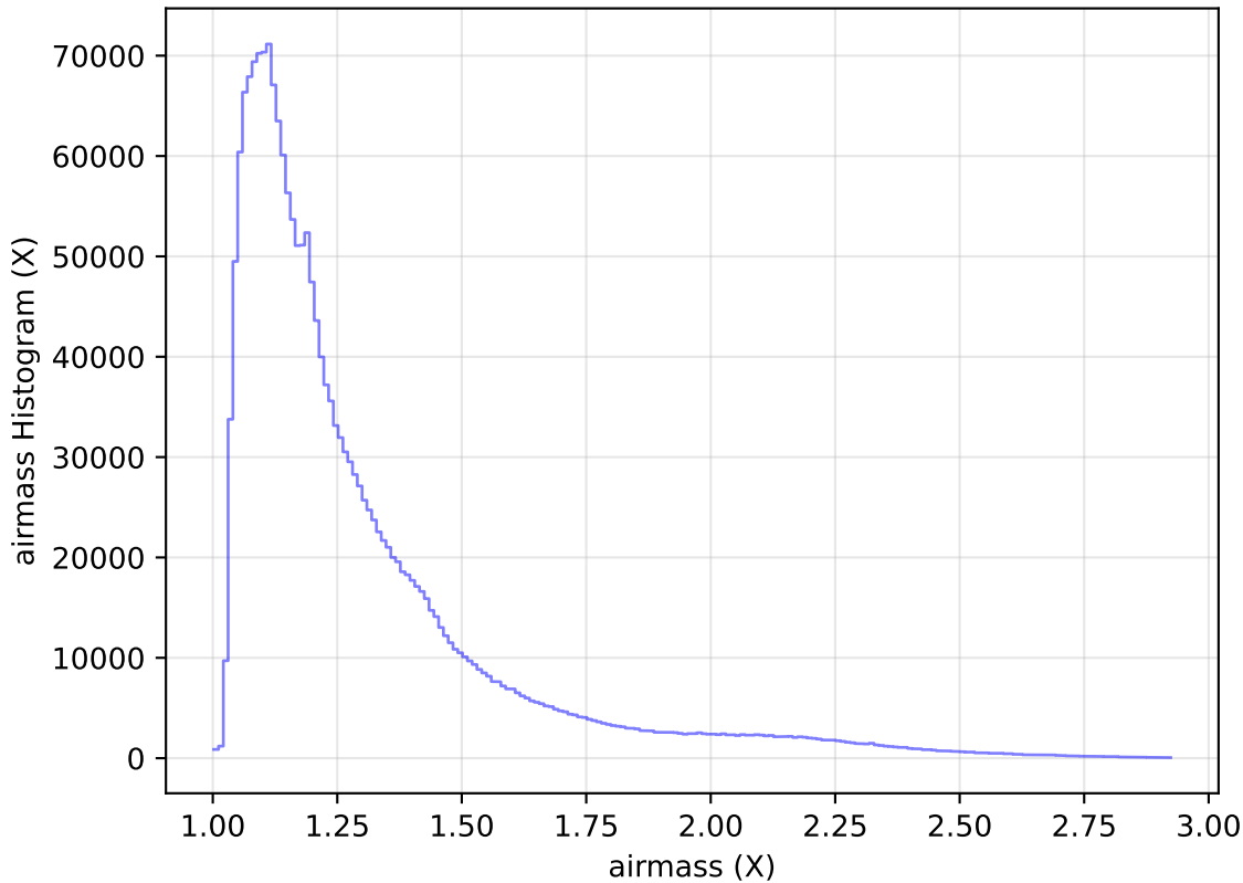
internal_u_expt38_nscale1.0v3.4_10yrs All sky all bands: airmass Histogram
