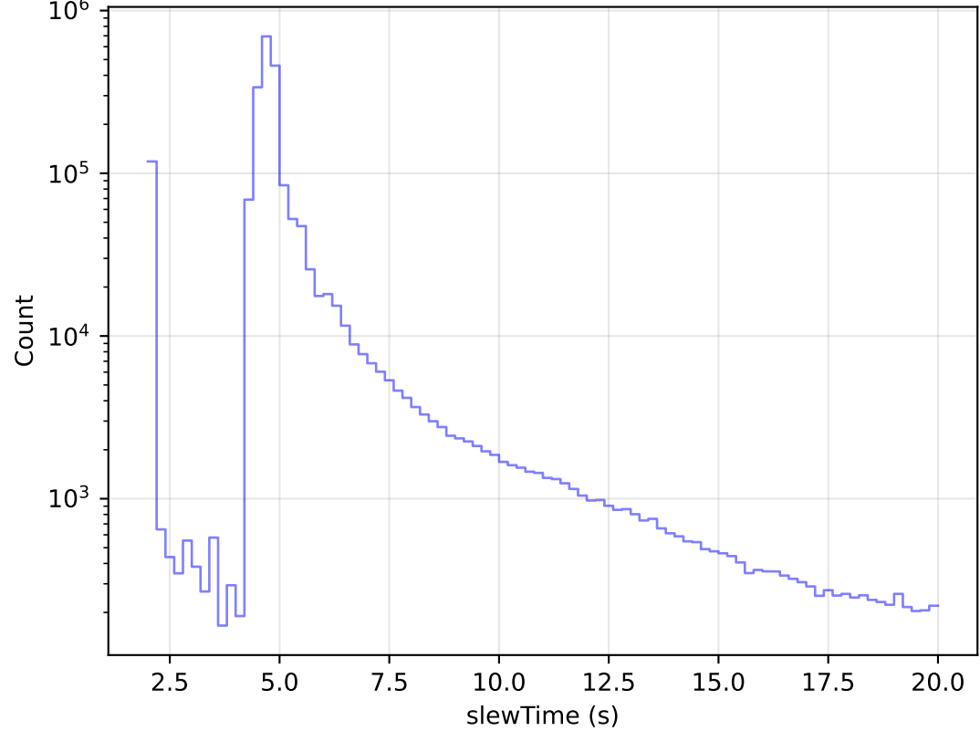
internal_u_expt38_nscale1.0v3.4_10yrs All visits: Zoom Slew Time Histogram
