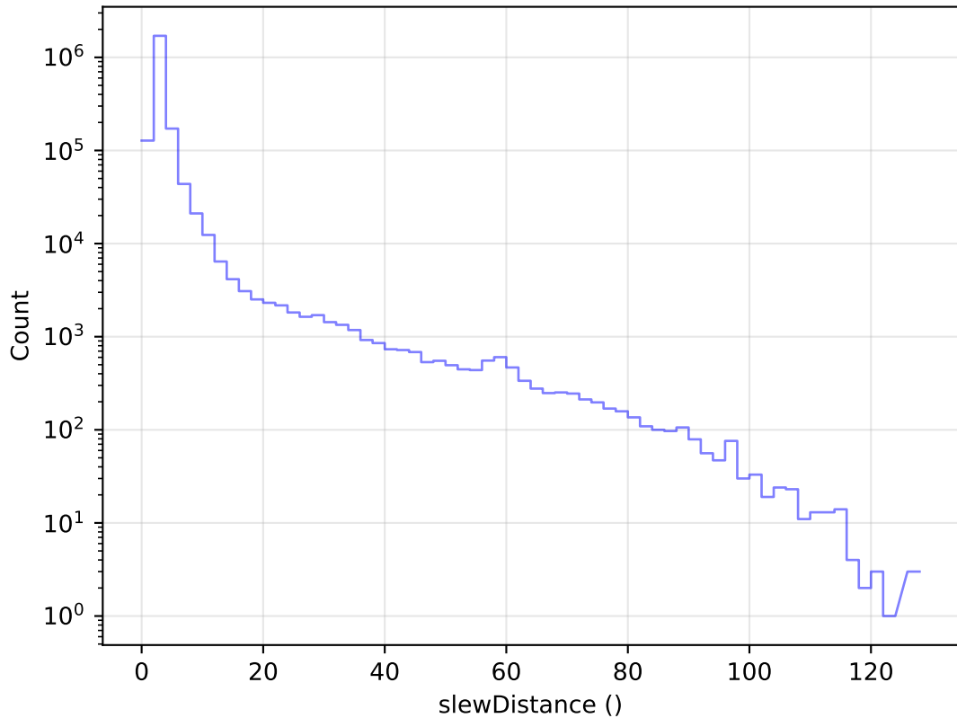
internal_u_expt38_nscale1.0v3.4_10yrs All visits: Slew Distance Histogram
