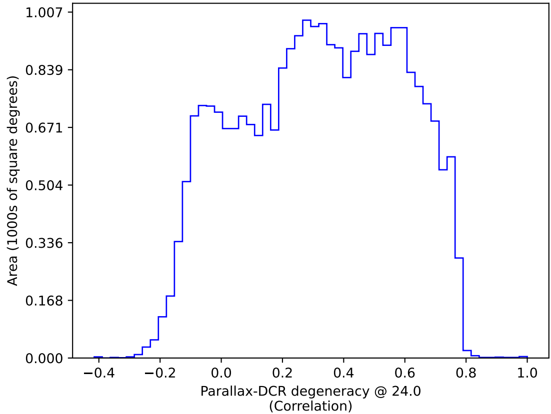
internal_u_expt38_nscale1.0v3.4_10yrs All sky: Parallax-DCR degeneracy @ 24.0
