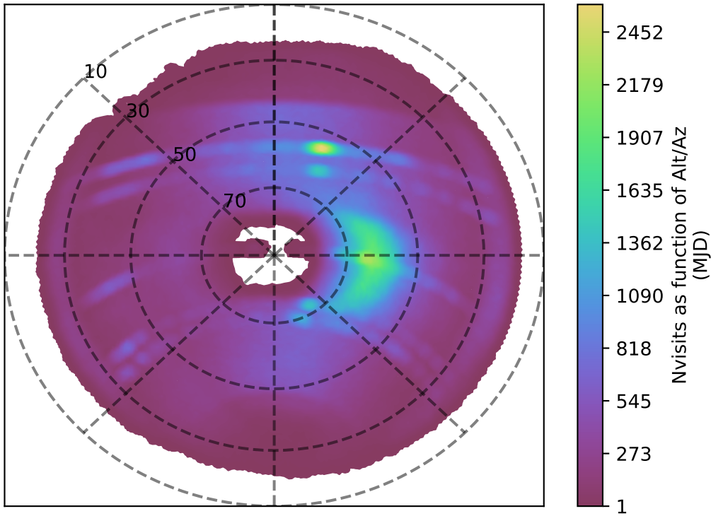
internal_u_expt38_nscale1.0v3.4_10yrs z band: Nvisits as function of Alt/Az
