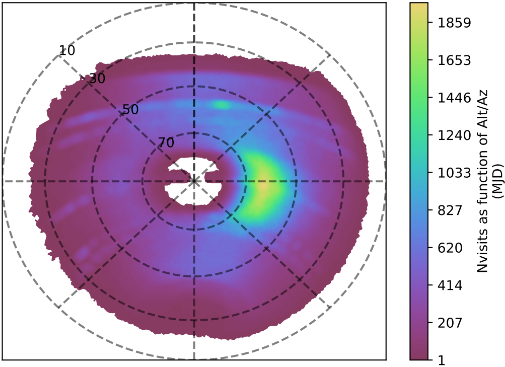
internal_u_expt38_nscale1.0v3.4_10yrs y band: Nvisits as function of Alt/Az
