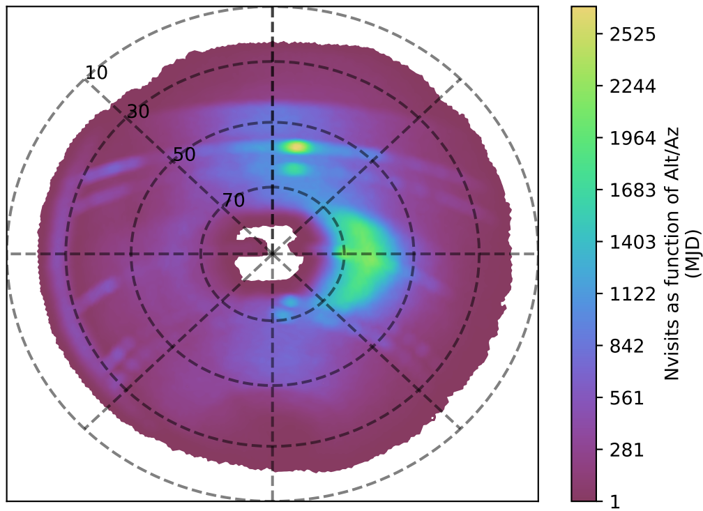
internal_u_expt38_nscale1.0v3.4_10yrs r band: Nvisits as function of Alt/Az
