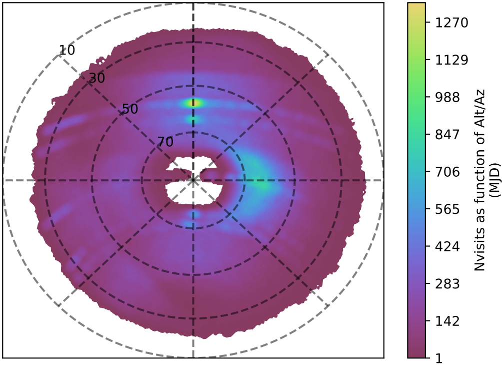
internal_u_expt38_nscale1.0v3.4_10yrs g band: Nvisits as function of Alt/Az
