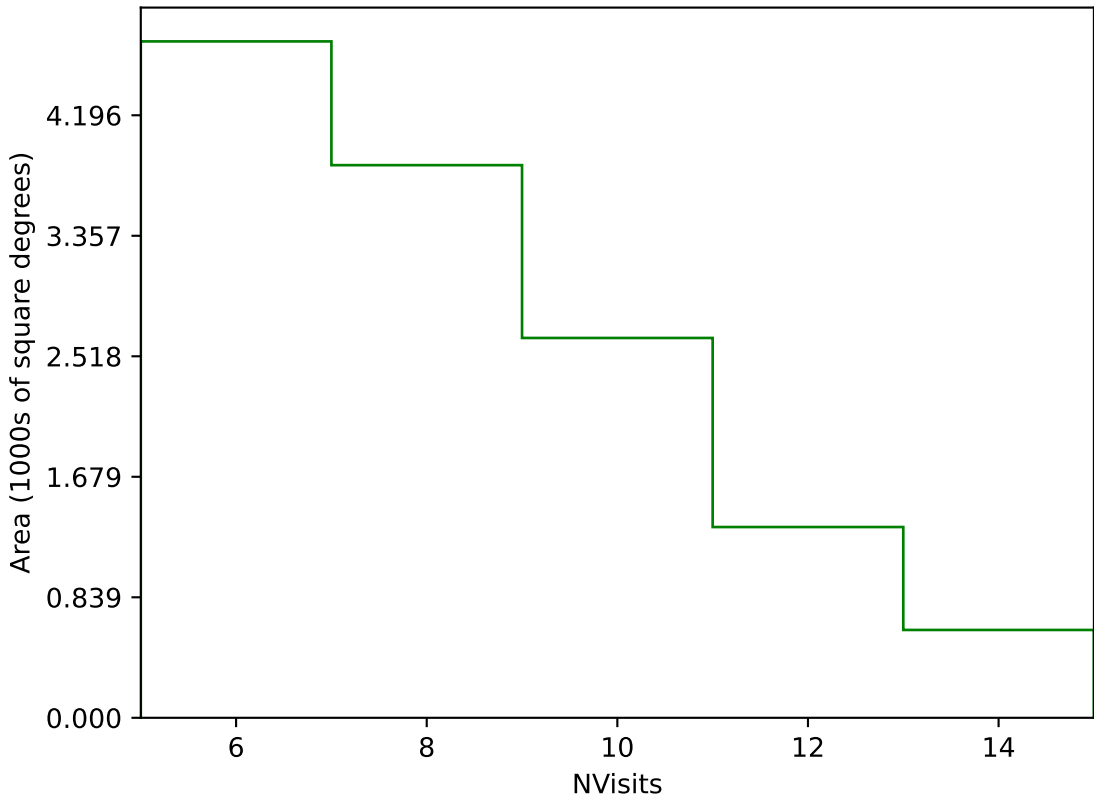
internal_u_expt38_nscale1.0v3.4_10yrs Yr 3-4 g band: NVisits
