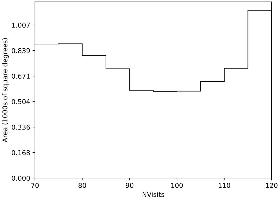
internal_u_expt38_nscale1.0v3.4_10yrs Yr 3-4 all bands: NVisits
