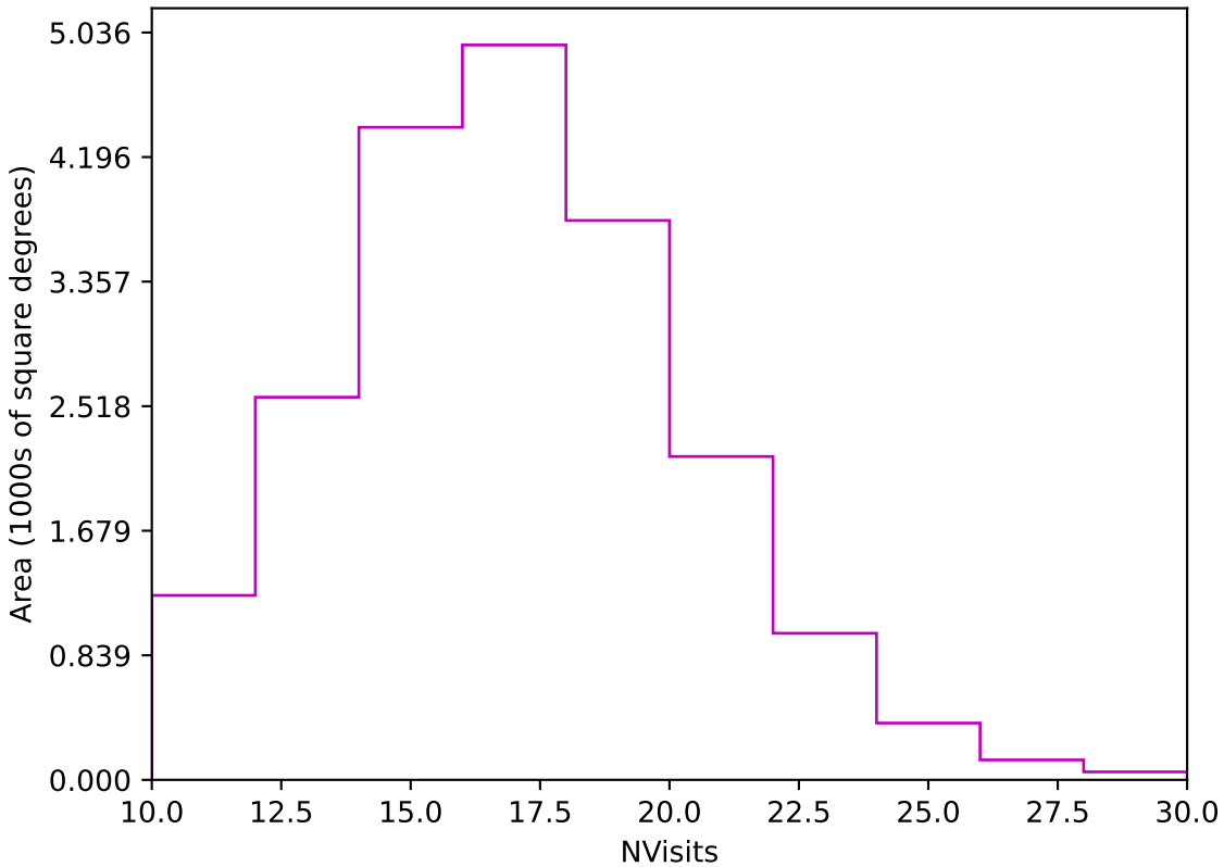
internal_u_expt38_nscale1.0v3.4_10yrs Yr 1 z band: NVisits
