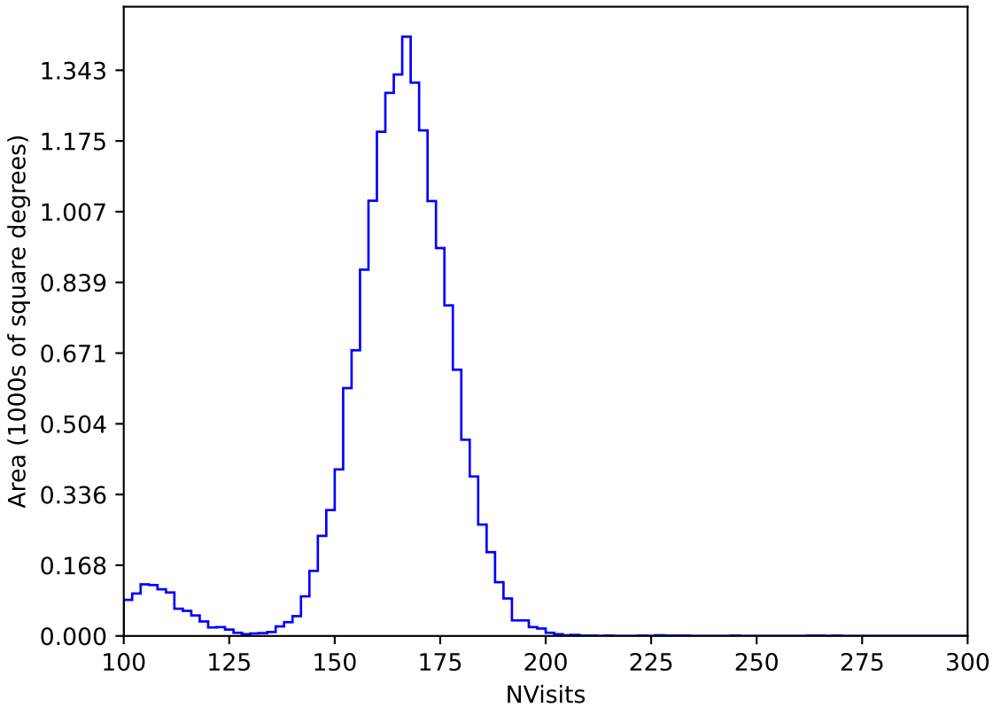
internal_u_expt38_nscale1.0v3.4_10yrs WFD y band: NVisits
