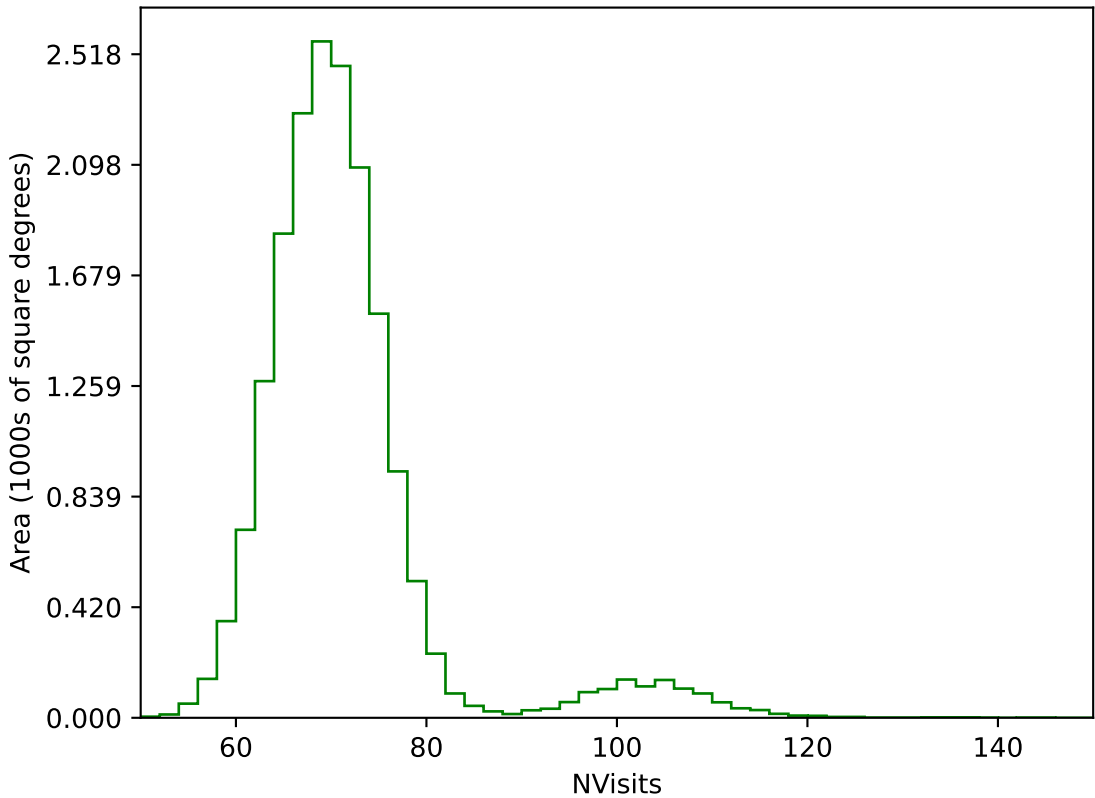
internal_u_expt38_nscale1.0v3.4_10yrs WFD g band: NVisits
